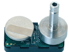
dV-1 OEM module with soldered-in battery and pressure sensor connection, ø 5 mm
